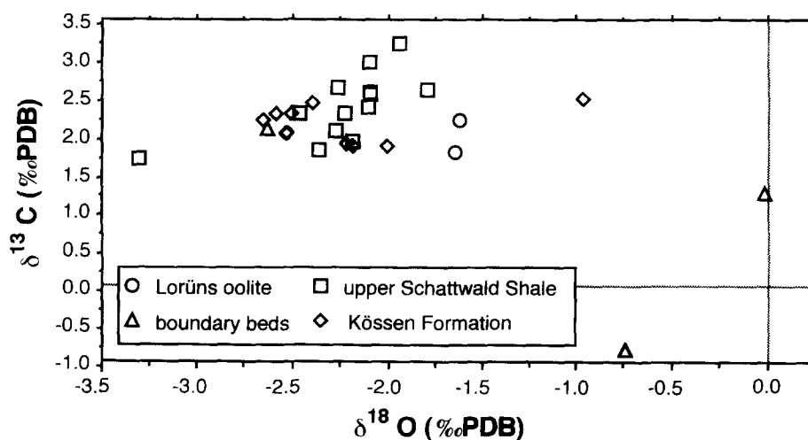
Fig. 6. Scatter plot of \delta^{13}\text{C} and \delta^{18}\text{O} values for samples across the Triassic–Jurassic boundary.
