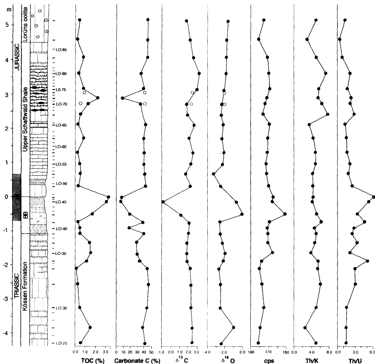
Fig. 5. Geochemical data from the Lorüns section. Note: circles represent measurements taken from the nodules presumed to be reworked from the underlying Kössen Formation. Cps = counts per second. See Fig. 3 for lithologic key.
