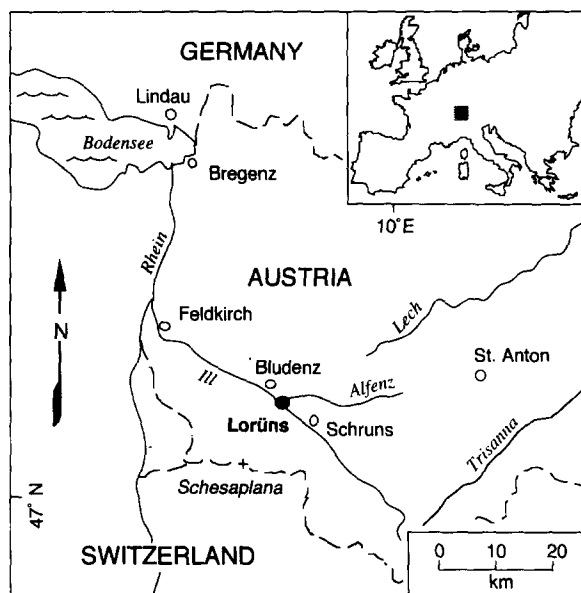
Fig. 1. Map of Vorarlberg region of western Austria showing the Lorüns quarry locality about 5 km southeast of Bludenz at the confluence of the Alfenz and Ill Rivers.
