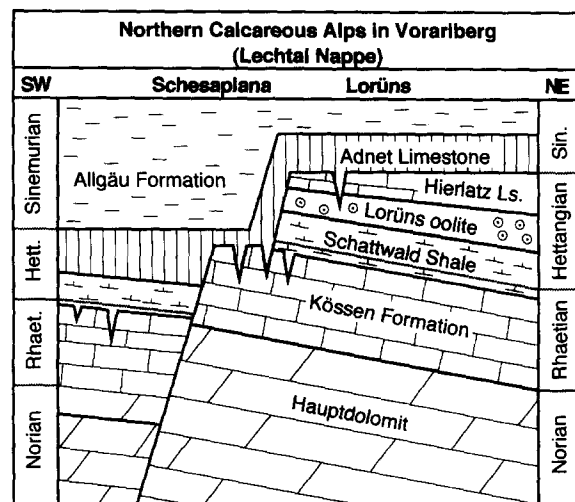
Fig. 2. Simplified regional Upper Triassic–Lower Jurassic stratigraphy of the Vorarlberg region of the Northern Calcareous Alps. The Lorüns area represents an isolated platform high and shows an expanded shallow-water platform sequence which contains fissure fillings within Lorüns oolite, containing clasts of Hierlatz Limestone. Near Schesaplana, about 12 km to the southwest of Lorüns, the Schattwald Shales and younger Jurassic deep-water sediments rest on top of or are contained within, fissure fills within the Rhaetian Kössen Formation. Modified from Furrer (1993).
