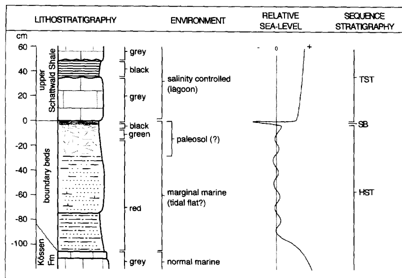
Fig. 7. Expanded view of boundary beds and local paleoenvironmental interpretation. See Fig. 3 for lithologic key. HST =highstands system tract; SB =sequence boundary; TST =transgressive systems tract.
